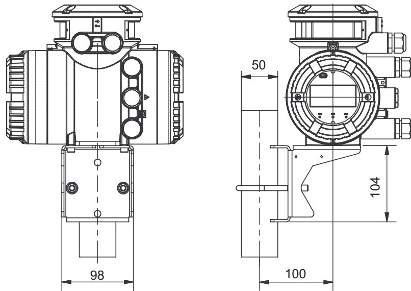
Fig. 32: Dimensions of transmitter in mm, attached by sheet metal console (bracket)
