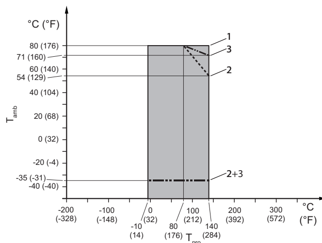
Fig. 25: Allowed process fluid and ambient temperatures, remote type for process connection type HS4 and HS8
