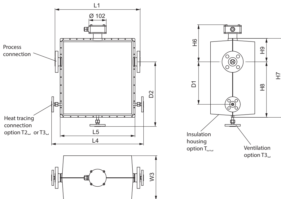
Fig. 30: Dimensions in mm: version with insulation housing
