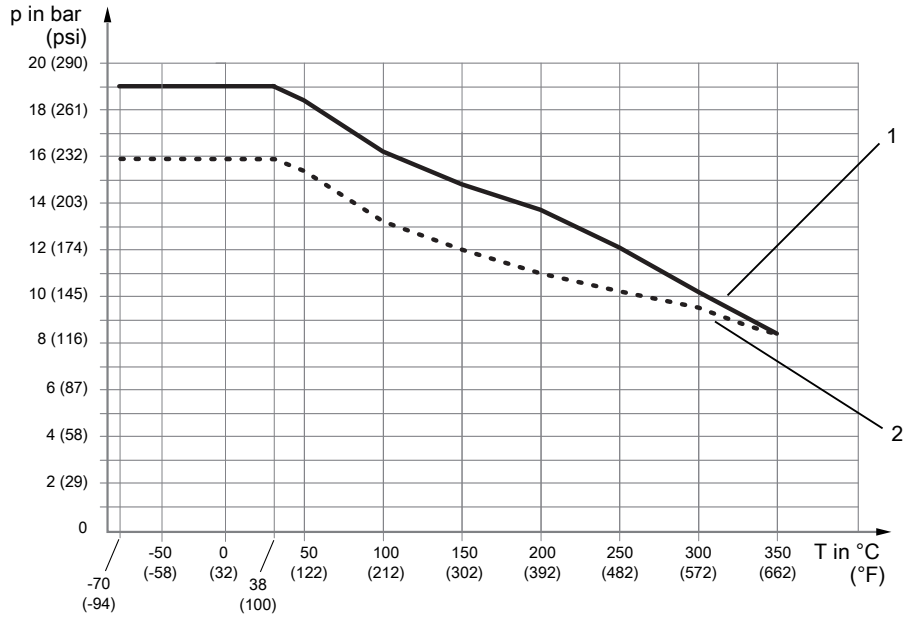
Fig. 13: Allowed process pressure as a function of process connection temperature
