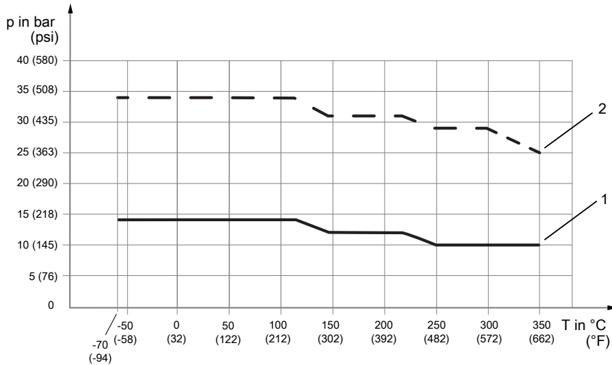
Fig. 17: Allowed process pressure as a function of process connection temperature
