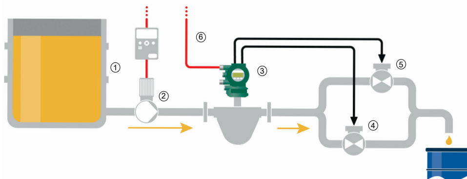
Fig. 50: Two-stage mode (The above diagram illustrates the fundamental functionality for one of several combination possibilities)
