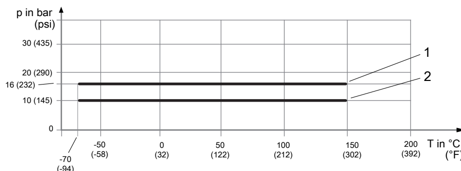
Fig. 20: Allowed process pressure as a function of process connection temperature
