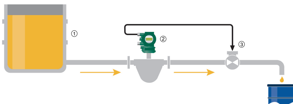
Fig. 49: One-stage mode (The above diagram illustrates the fundamental functionality for one of several combination possibilities)
