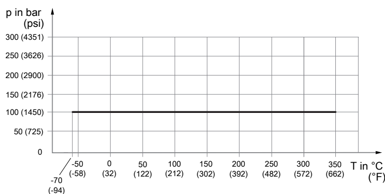
Fig. 21: Allowed process pressure as a function of process connection temperature
