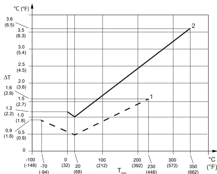
Fig. 11: Temperature accuracy
