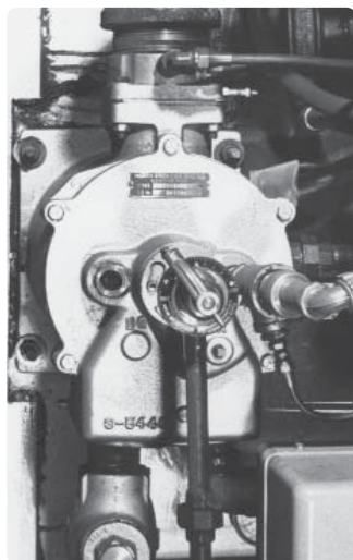
1813 Sensitrol Valve on a Dual-Fuel™ burner. Valve is used for setting ratio when burner is on oil; it is shut off when burning gas.
