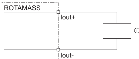
Fig. 19: Active current output connection lout HART
