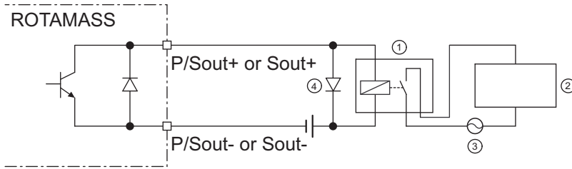
Fig. 32: Passive status output connection P/Sout or Sout for solenoid valve circuit
