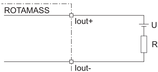
Fig. 21: Passive current output connection I out
