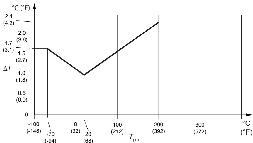
Fig. 5: Temperature accuracy
