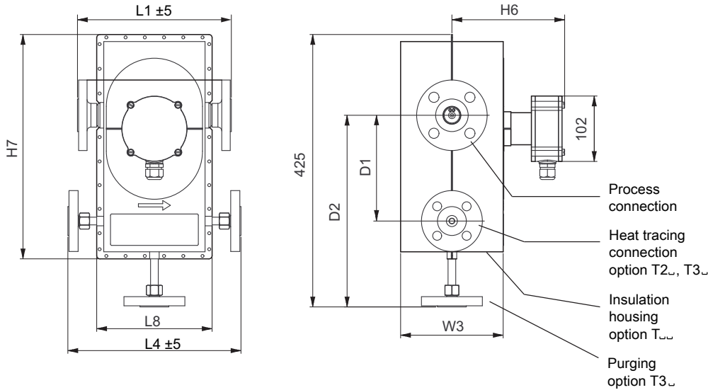
Fig. 23: Dimensions in mm: version with insulation housing
