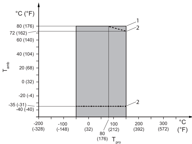
Fig. 17: Allowed process fluid and ambient temperatures, remote type (except process connection type HS4 and HS8)
