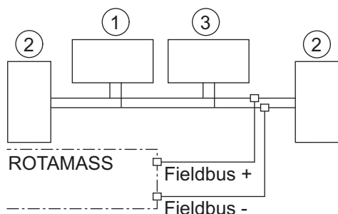
Fig. 43: FOUNDATION Fieldbus connection
