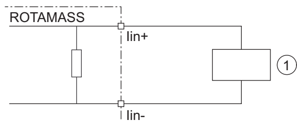
Fig. 30: Connection of external device with active current output
