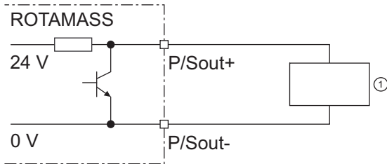
Fig. 33: Active pulse output P/Sout with internal pull-up resistor
