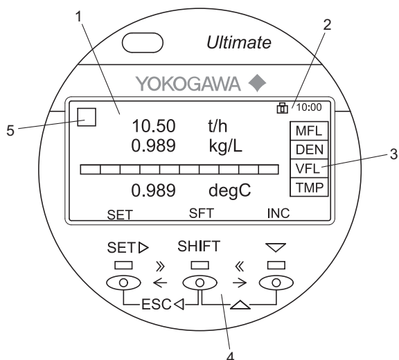
Fig. 44: Display layout
