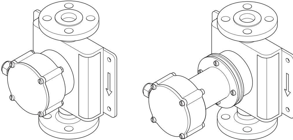
Fig. 20: Sensor with standard and long neck
