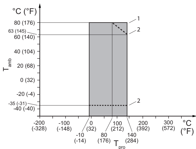
Fig. 18: Allowed process fluid and ambient temperatures, remote type for process connection type HS4 and HS8
