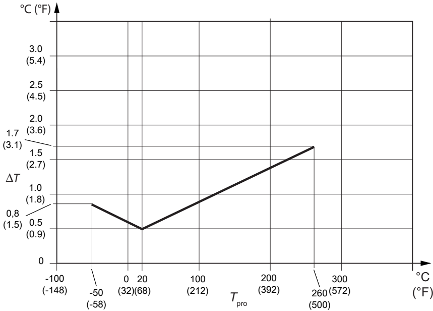
Fig. 5: Temperature accuracy
