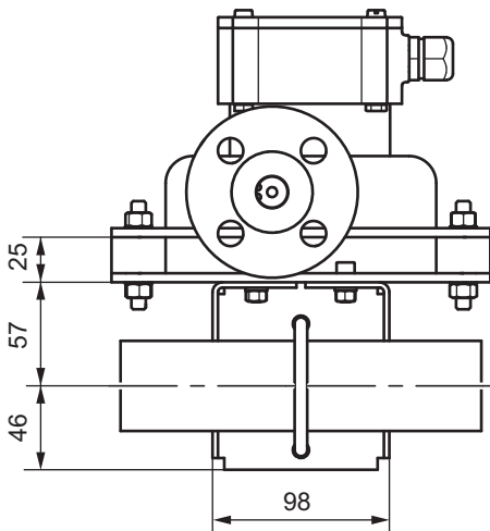
Fig. 22: Dimensions in mm: fixing device option PD for Nano
