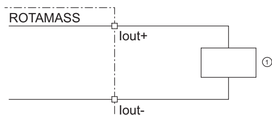
Fig. 26: Active current output connection lout HART
