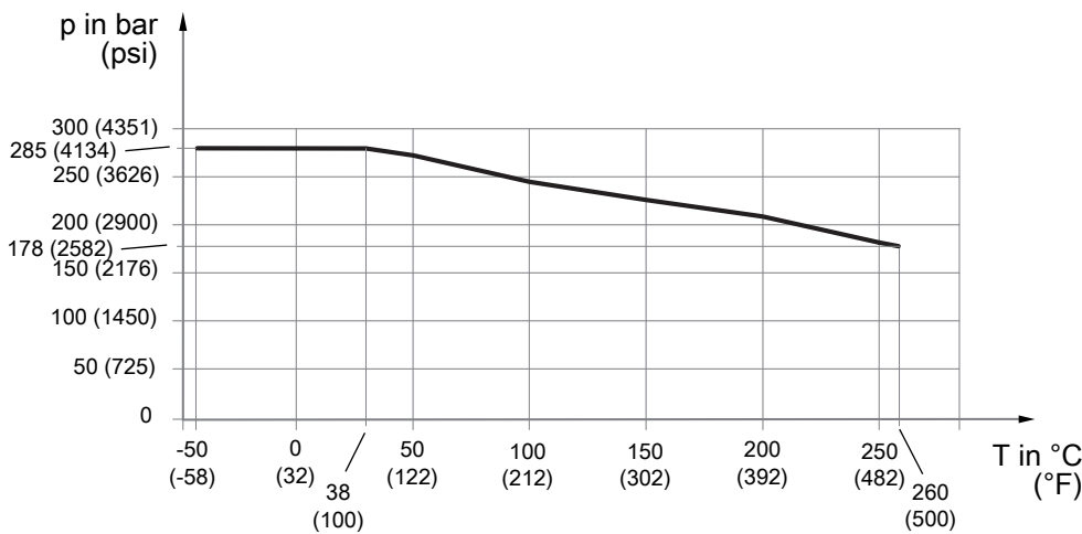
Fig. 15: Allowed process pressure as a function of process fluid temperature
