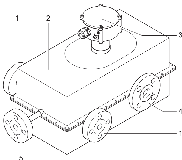
Fig. 16: Configuration of Rotamass with insulation and heat tracing
