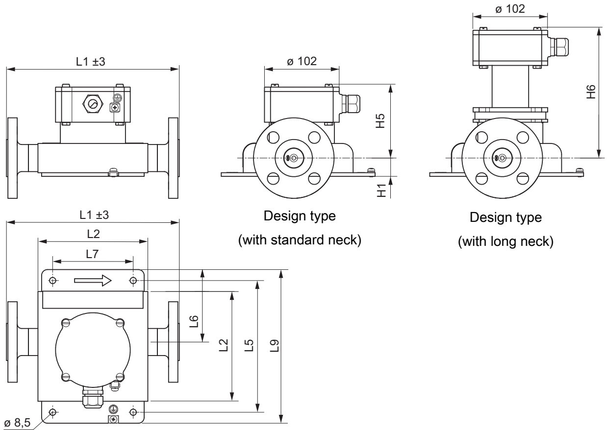
Fig. 21: Dimensions in mm
