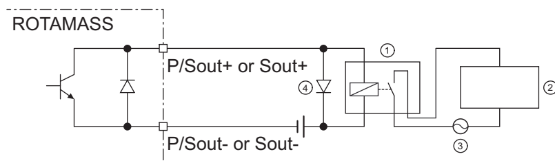
Fig. 39: Passive status output connection P/Sout or Sout for solenoid valve circuit
