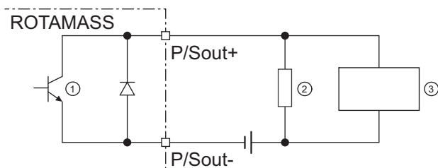
Fig. 34: Passive pulse output connection P/Sout with electronic counter
