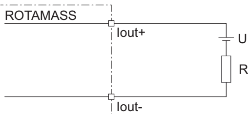
Fig. 28: Passive current output connection lout
