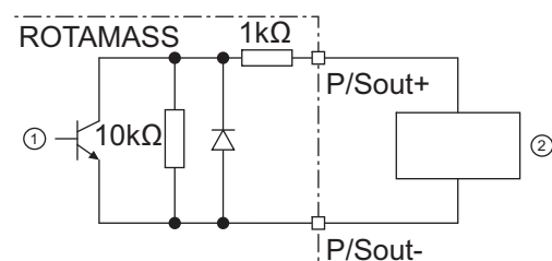
Fig. 40: Passive pulse or status output with switching amplifier connected in series
