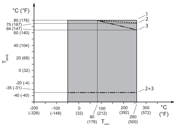
Fig. 19: Allowed process fluid and ambient temperatures
