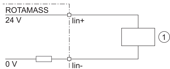
Fig. 29: Connection of external device with passive current output
