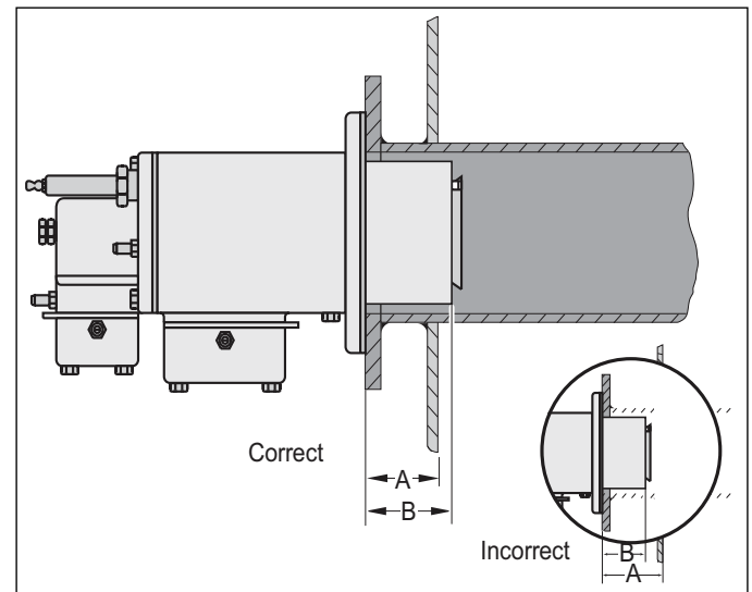
Figure 3.7. Air Tube Length
