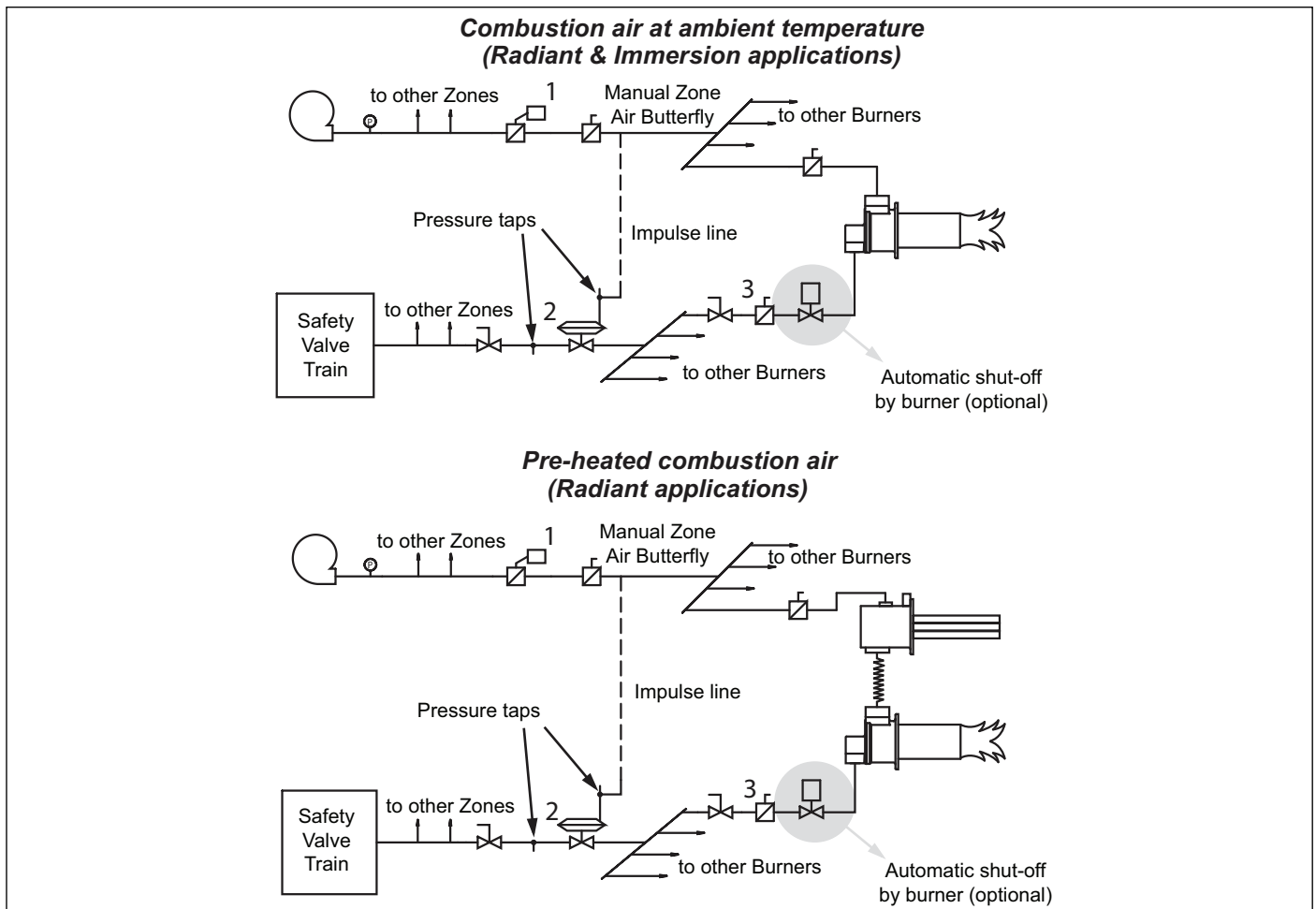
Figure 3.9. System Schematics
