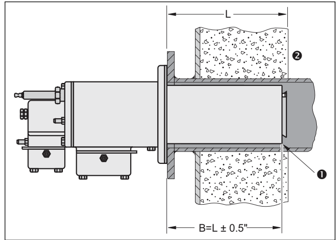
Figure 3.5. Air Tube Length
