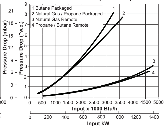
Loading Line Pressure vs. Input Measured at Tap "A"
