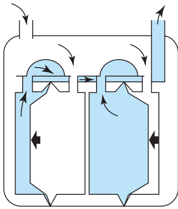
Working Principle
